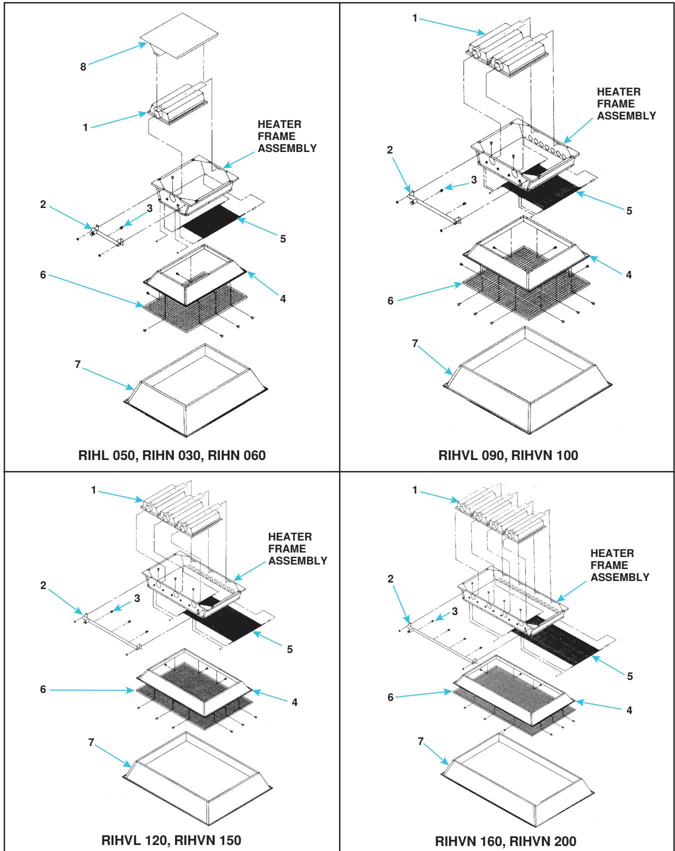
Figure 2. Heater Components (Refer to Table 2 )
