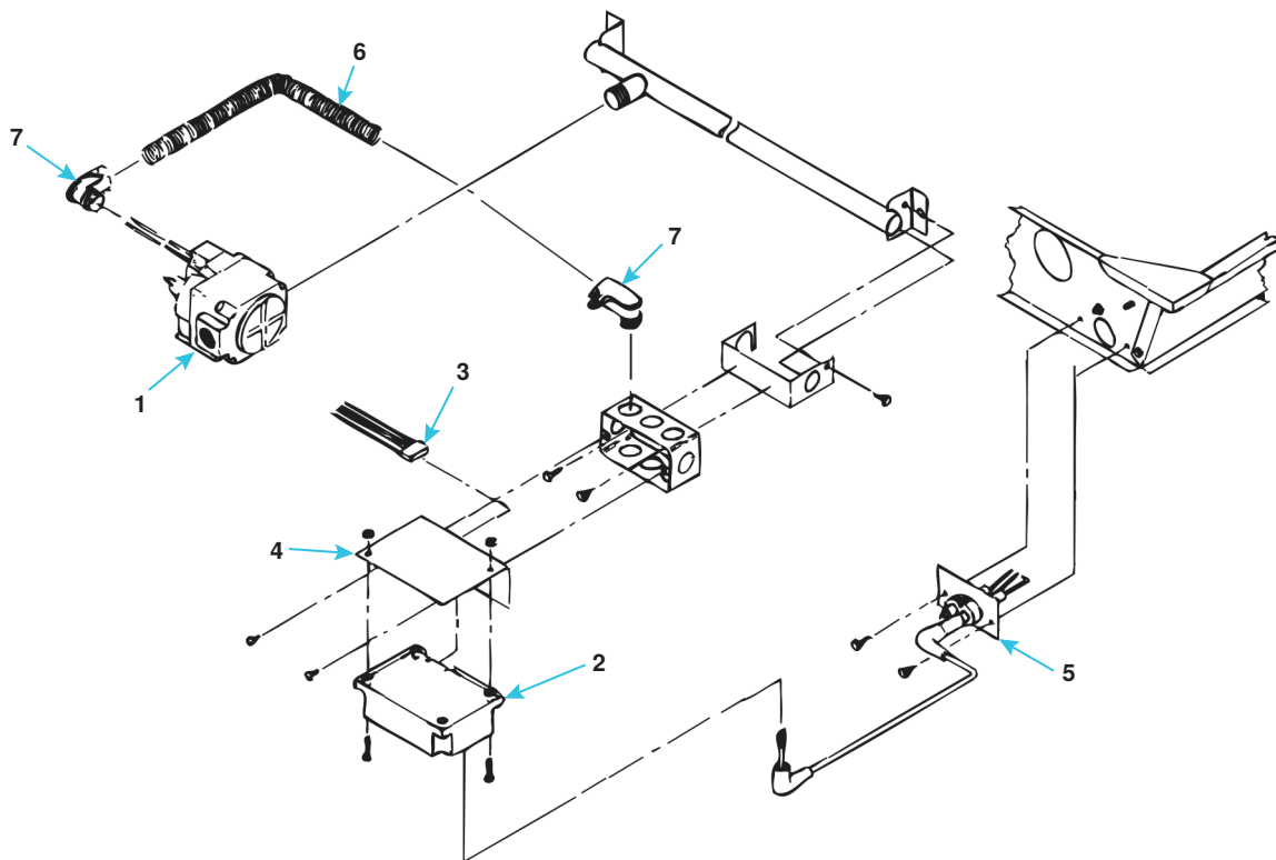
Figure 1. Control Components (Refer to Table 1 )
