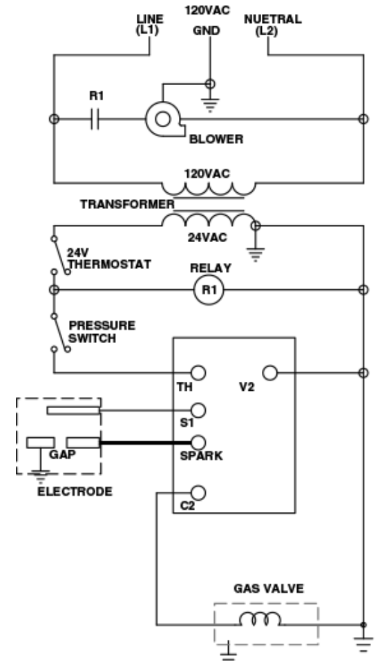
LADDER DIAGRAM
