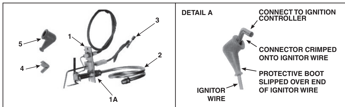
Figure 7. Horizontal Spark Pilot Replacement Kit (Refer to Table 10 )
