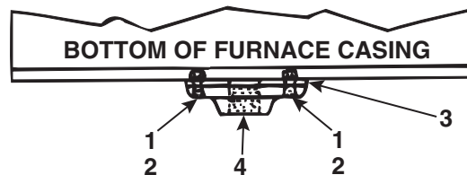
Figure 10. Condensate Drain Kit (Refer to Table 12 )
