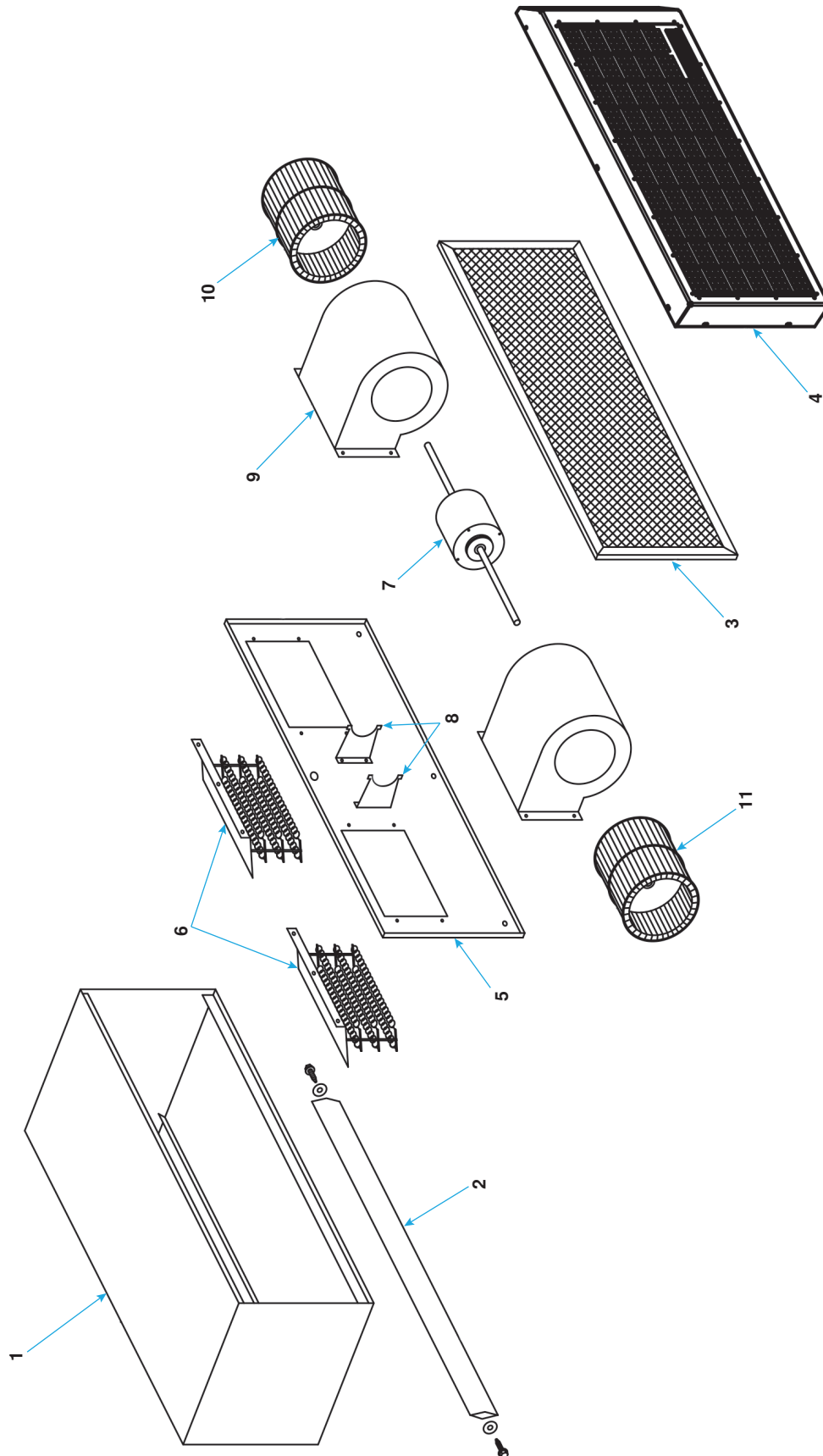
Figure 1. Typical Exploded View (Refer to Table 1 and Table 2 )
