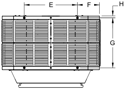
Figure 3 Minimum Clearances
