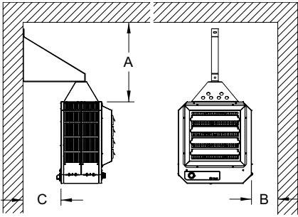
Figure 2 Threaded Rod Spacing Dimensions Horizontal Air Discharge
