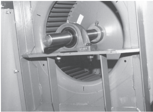
Figure 24. Blower Motors and Bearings—RGLB, RPBL, and PGBL Model BL-Type Blower Cabinets (Refer to Table 48 )
