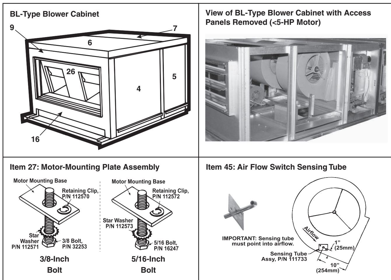
Figure 23. RGBL, RPBL, and PGBL Model BL-Type Blower Cabinet Section Components (Refer to Table 48)
