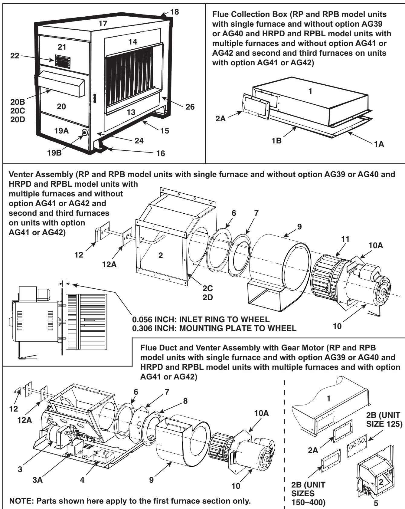
Figure 12. RP Model Collection Box Components (Refer to Table 19 )
