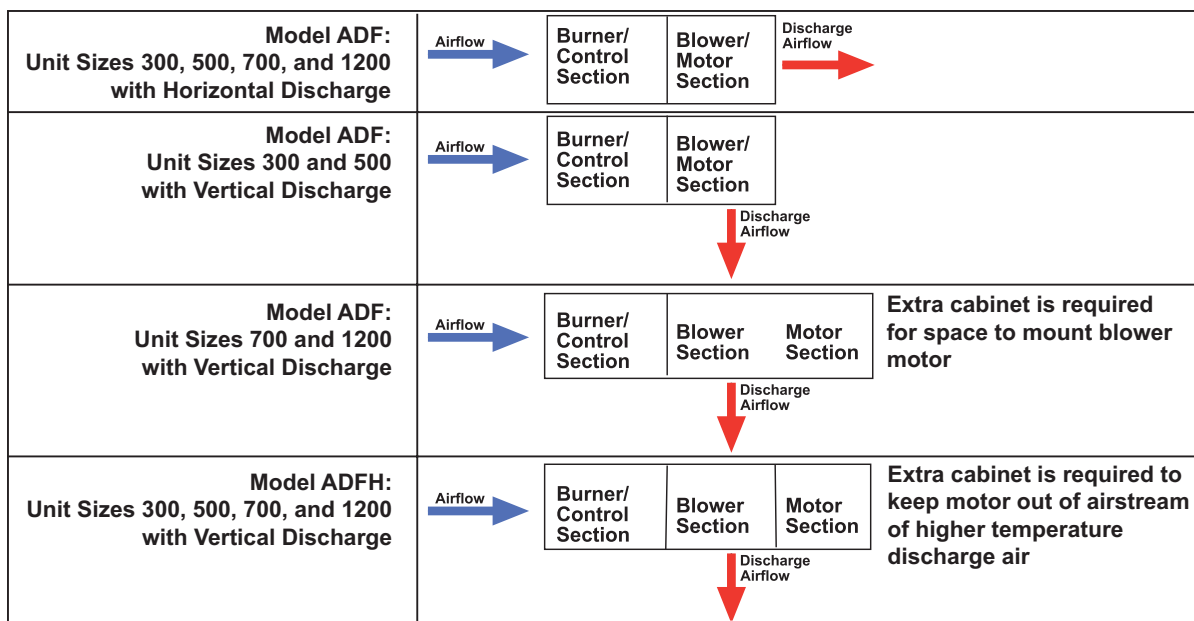
Figure 1. Cabinet Configurations
