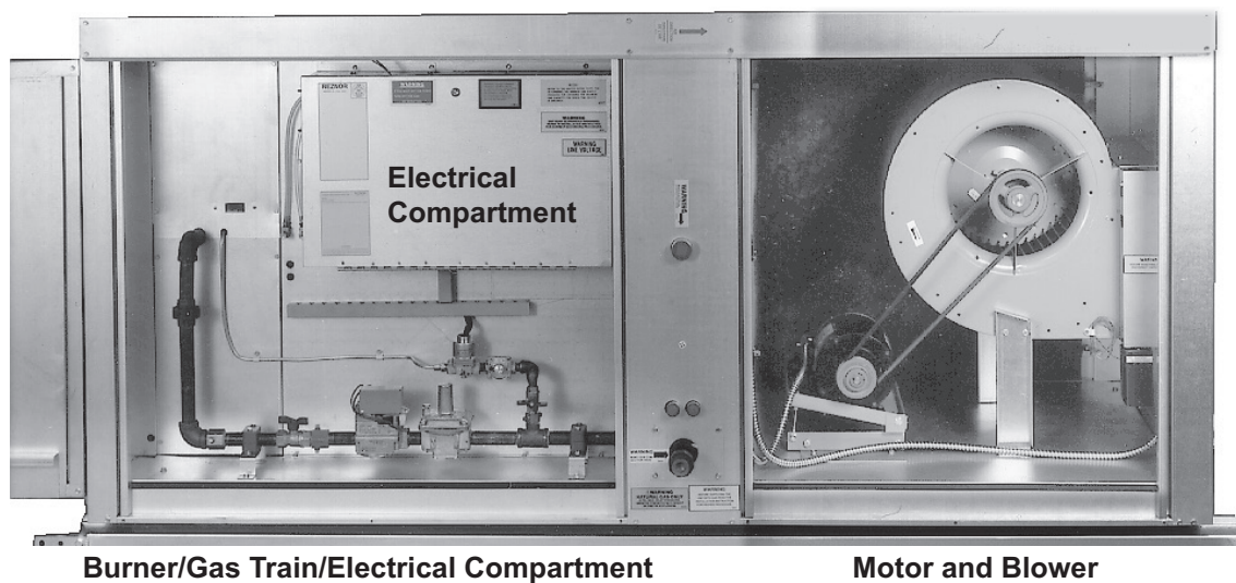
Figure 2. Cabinet Compartments (Refer to Table 2 )
