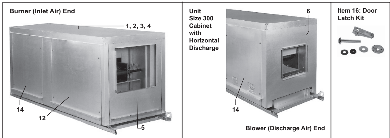
Figure 14. Cabinet Components (Refer to Table 22)
