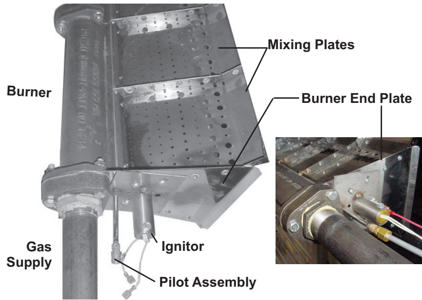
Figure 11. Burner Assembly for Units Manufactured after AUG 2003 (Refer to Table 16 )
