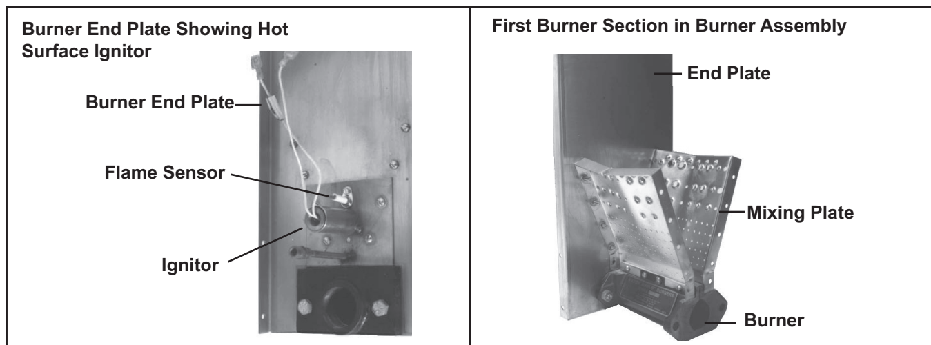
Figure 10. Burner Assembly for Units Manufactured Before SEP 2003 (Refer to Table 15 )
