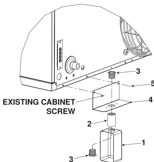
Figure 1. Typical Thermostat Bracket Kit (Refer to Table 1)
