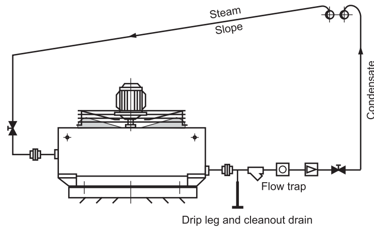
Vertical Discharge Units
