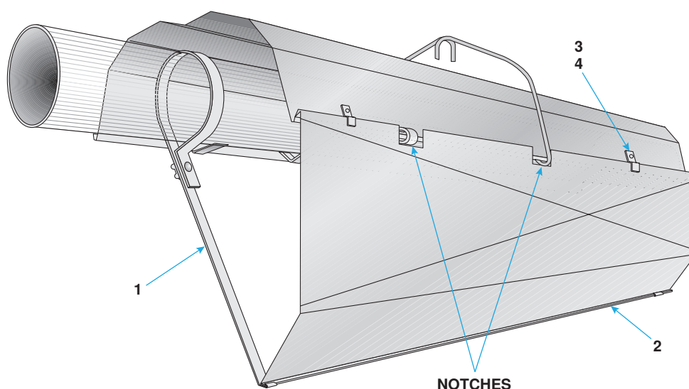
Figure 1. Reflector Side Extension Installation (Refer to Table 1)
