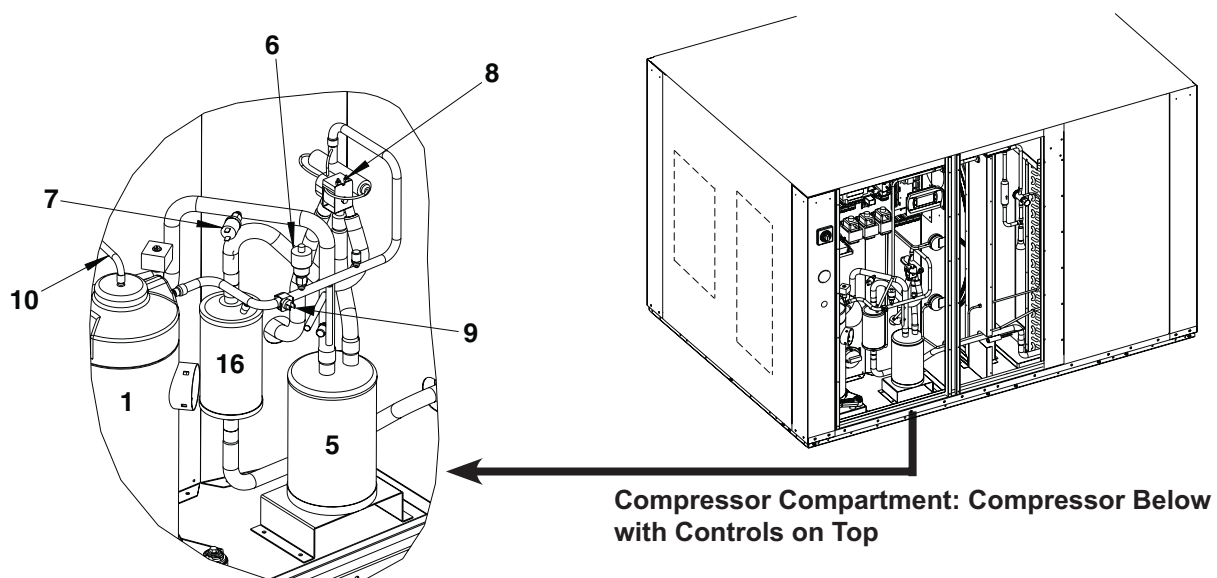
Figure 11. Compressor Compartment Components (Refer to Table 10 )
