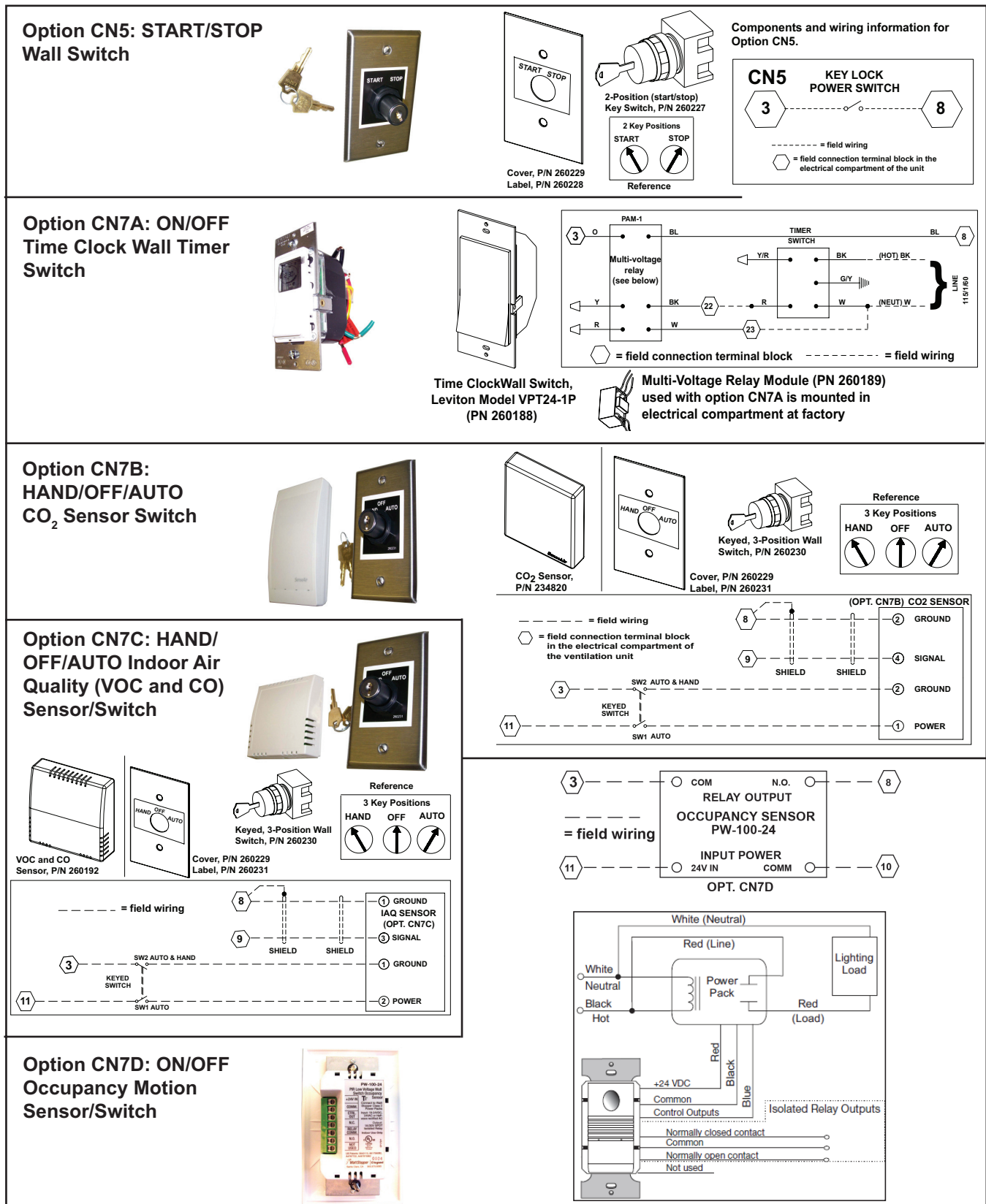
Figure 3. Occupancy Control Options (Refer to Table 3 )
