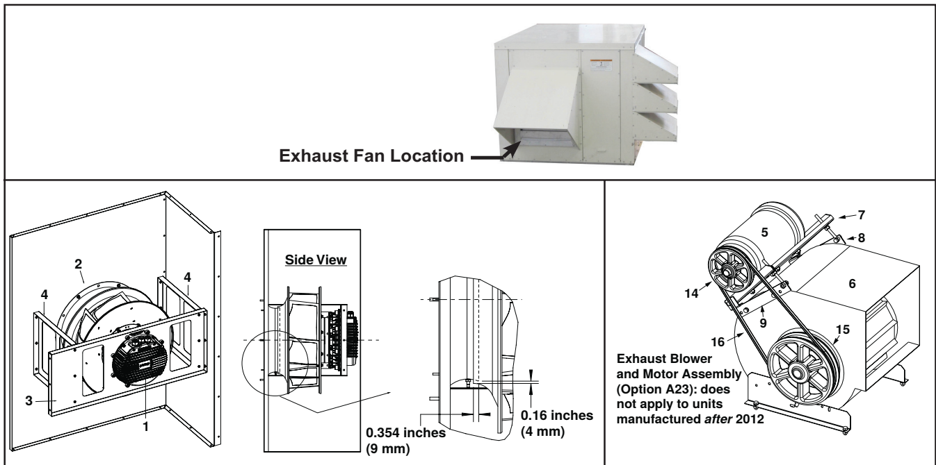
Figure 10. Exhaust Fan Assembly (Refer to Table 9 )
