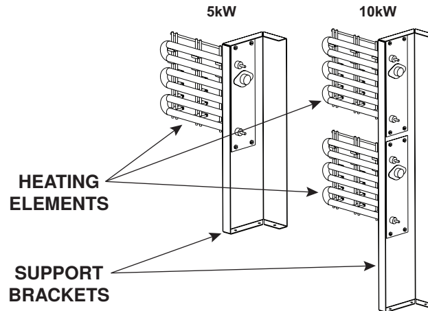
Figure 6. Optional Electric Pre-Heat Components (Refer to Table 5 )
