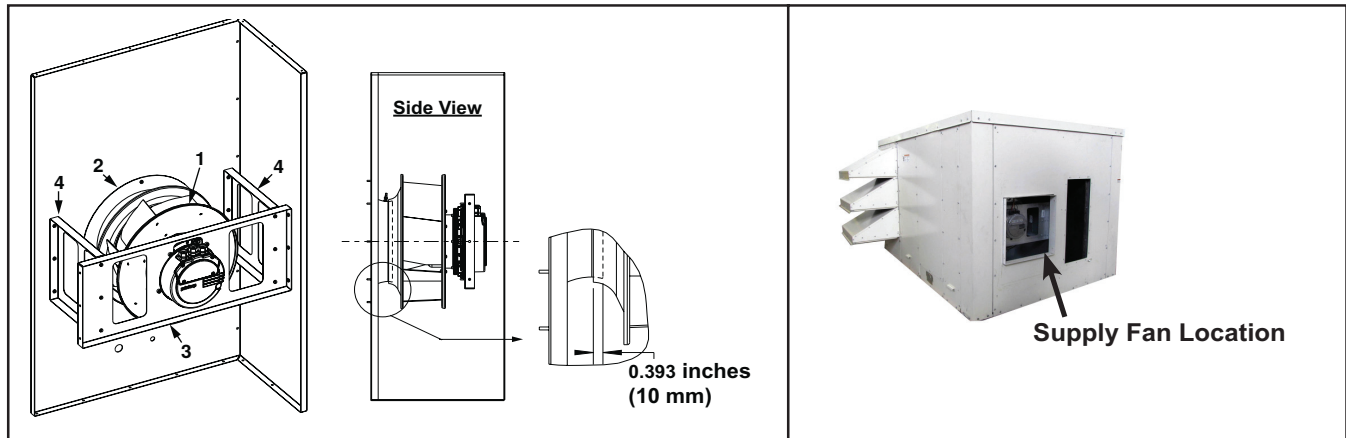
Figure 9. Supply Fan Assembly (Refer to Table 8 )
