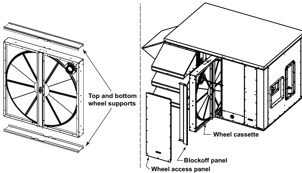
Figure 8. Energy Recovery Wheel Components (Refer to Table 7 )
