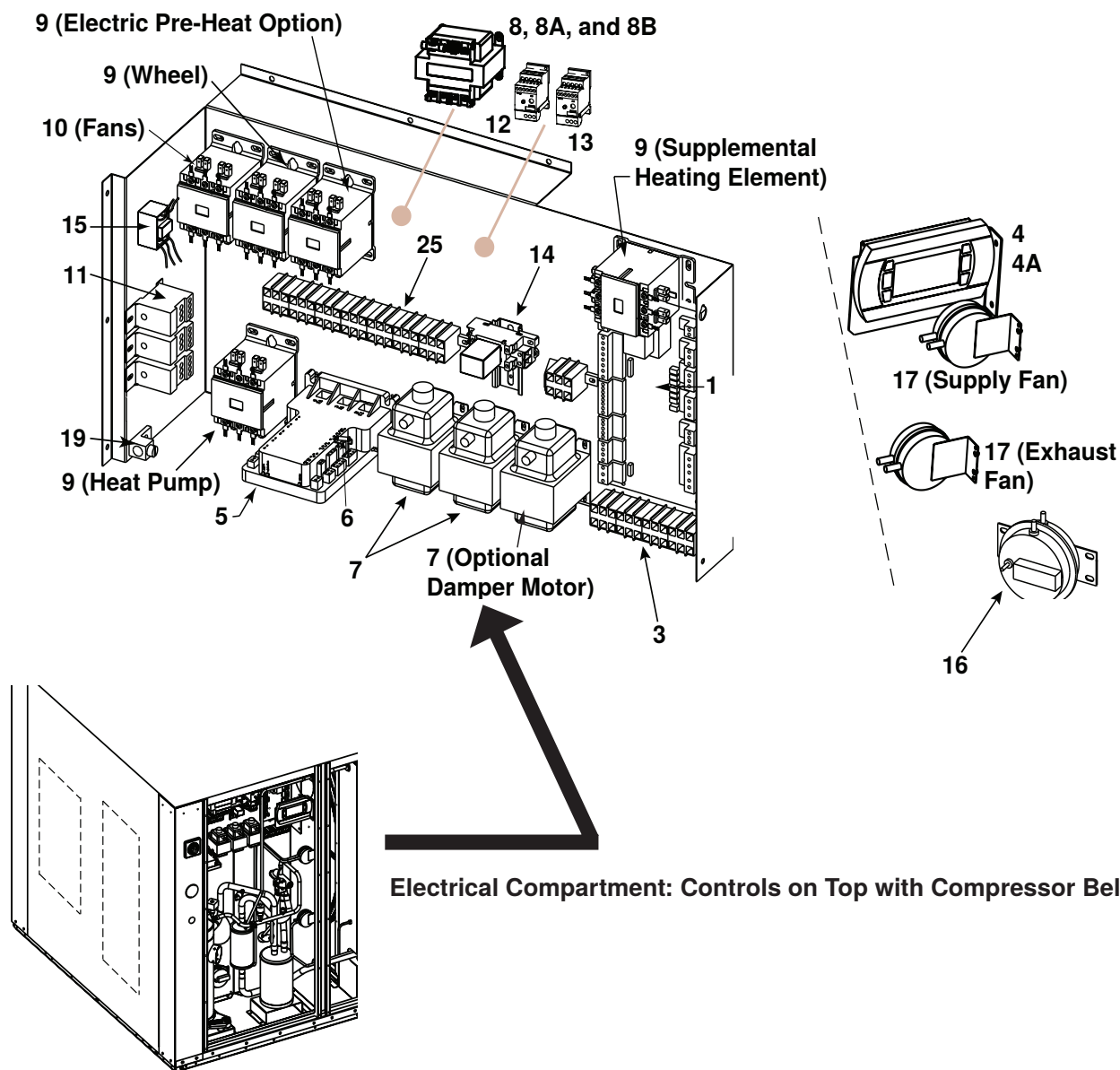
Figure 1. Electrical Compartment Components (Refer to Table 2 )
