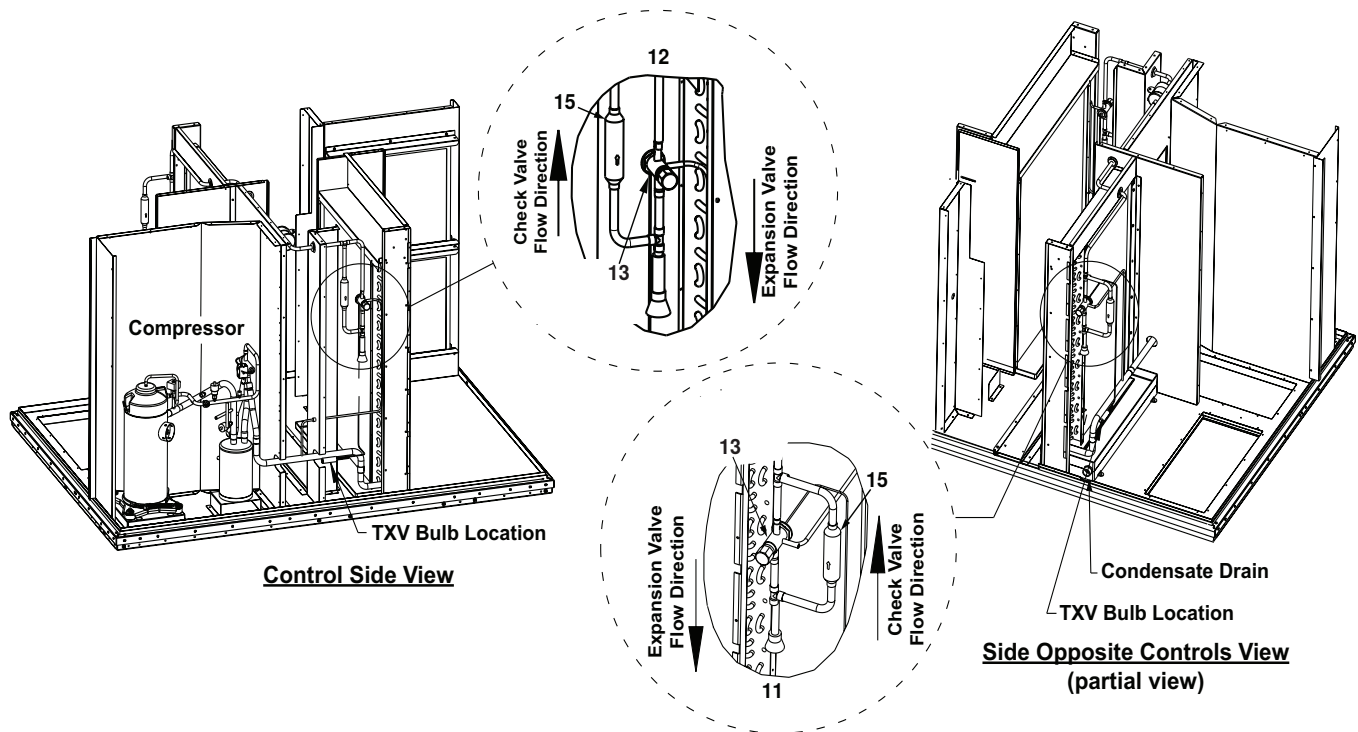
Figure 12. Coil Compartment Components (Refer to Table 10 )
