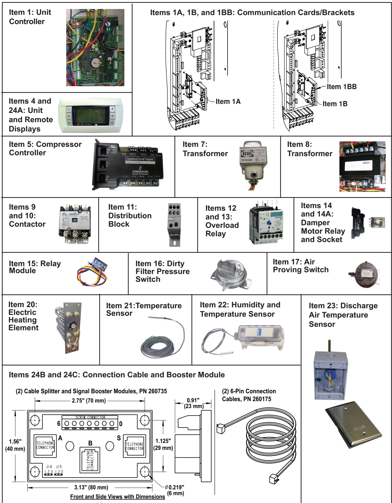
Figure 2. Individual Electrical Components (Refer to Table 2 )
