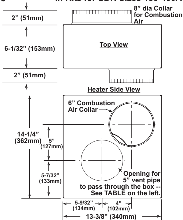
Concentric Adapter Box in Kits for SDH Sizes 150-400A
