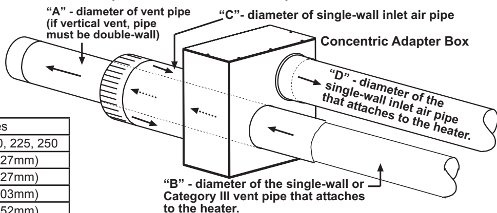
Model SDH 75, 100, 125, 175, 200, 225, and 250 - Pipe Diameters and Connections Required at the Concentric Adapter Box
