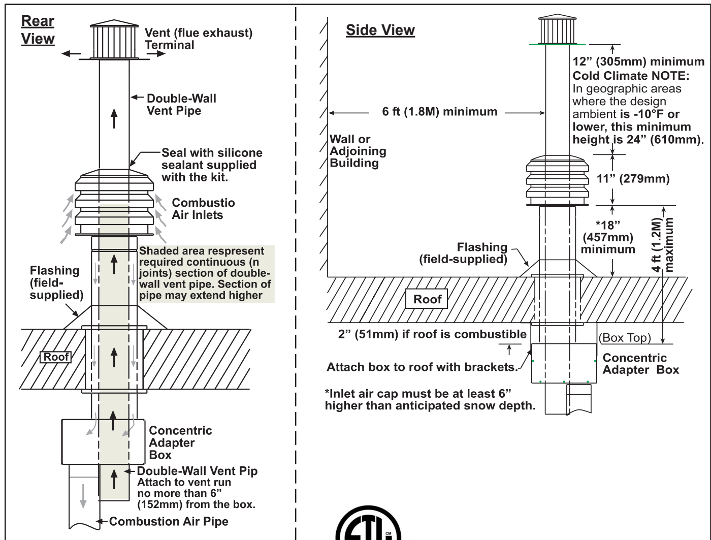
FIGURE 17 - Installation of Unit with Vertical Vent Terminal/ Combustion Air Inlet (Option CC2)
