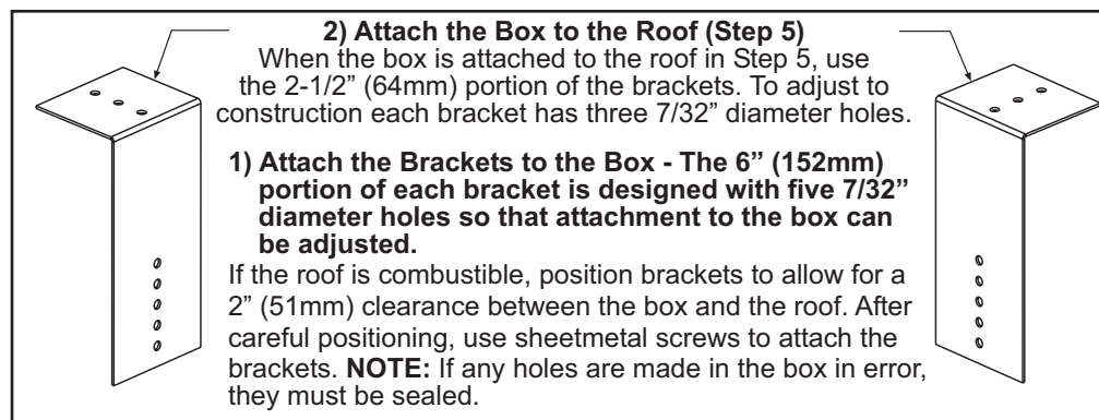
FIGURE 13 - Brackets for Attaching the Concentric Adapter Box to the Roof
