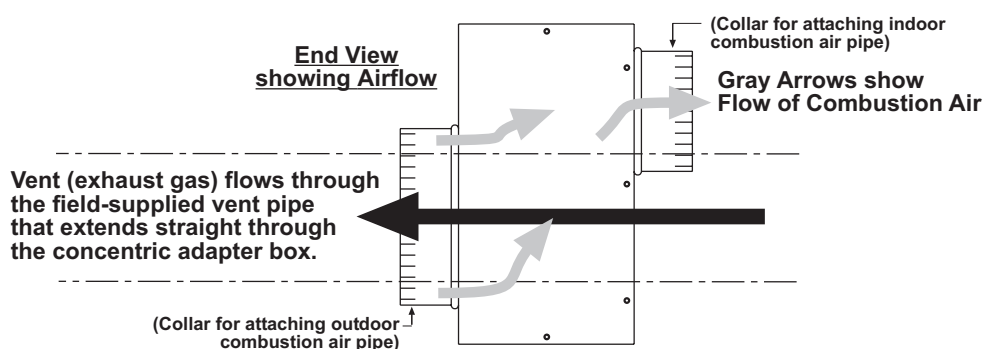
FIGURE 6 - Concentric Adapter Box Airflow
