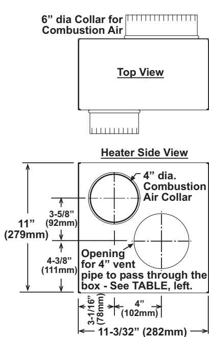
Concentric Adapter Box in Kits for SDH Sizes 75-125
