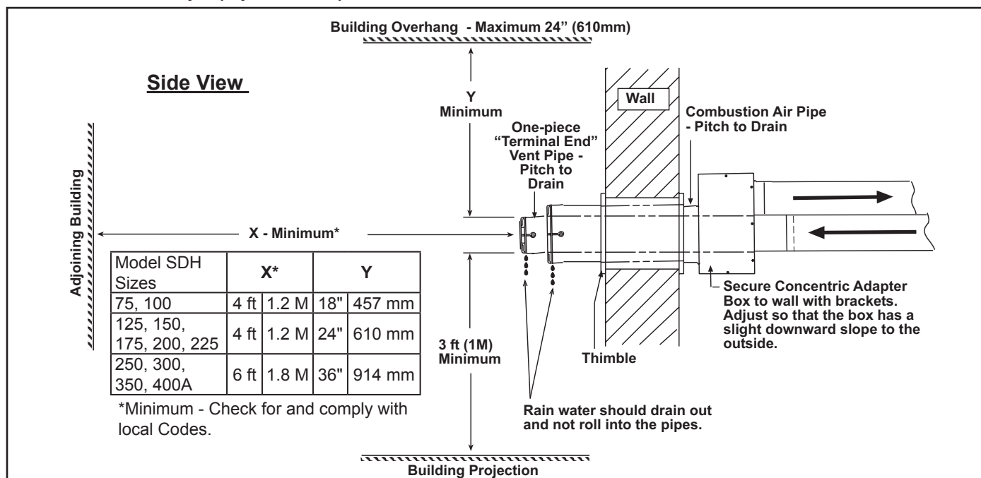
FIGURE 12 - Installation of a Typical Separated-Combustion Unit with Horizontal Vent Terminal and Combustion Air Pipe (Option CC6)
