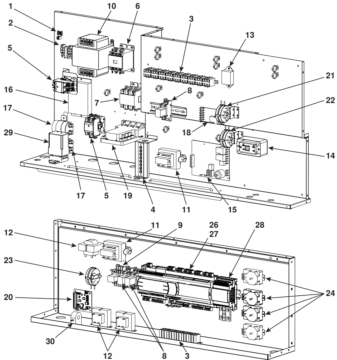
Figure 2. Main and Secondary Control Panels (Refer to Table 2 )
