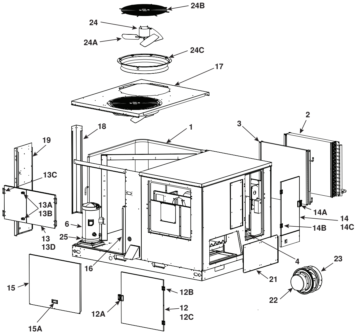
Figure 1. Main Cabinet Assembly (Refer to Table 1 )
