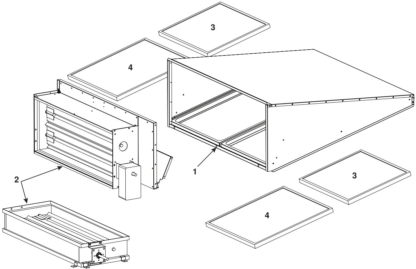
Figure 5. Economizer (Refer to Table 5 )
