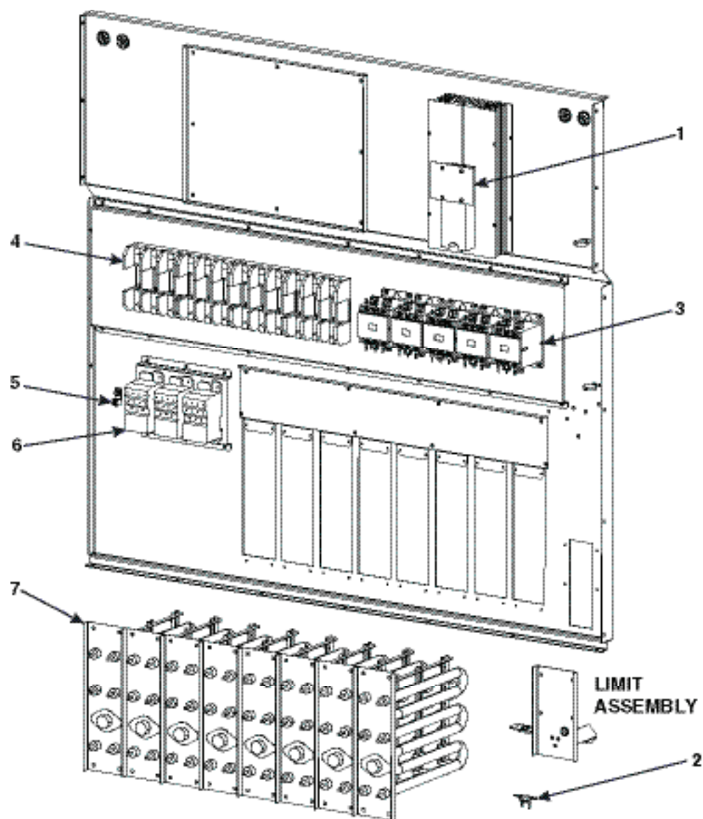
Figure 4. Electric Heat Section (Refer to Table 4 )
