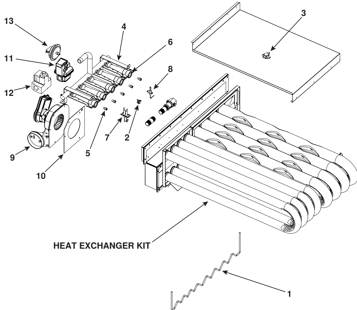
Figure 3. Gas Heat Section (Refer to Table 3 )
