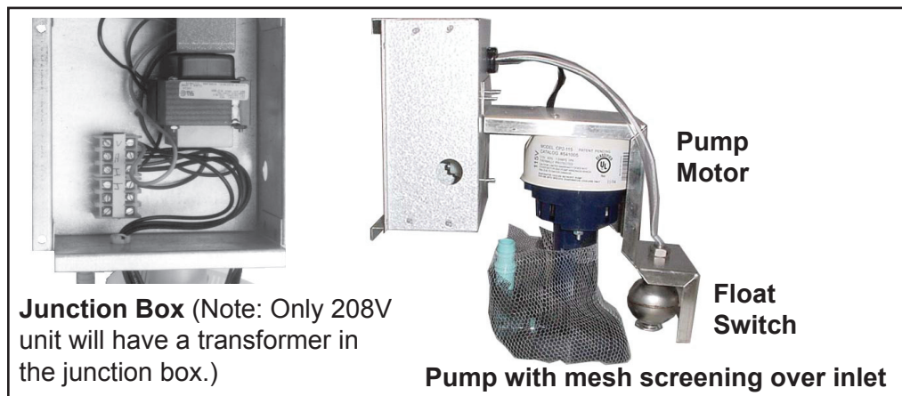
FIGURE 16 - Remove Junction Box, Pump and Float Switch as an Assembly
