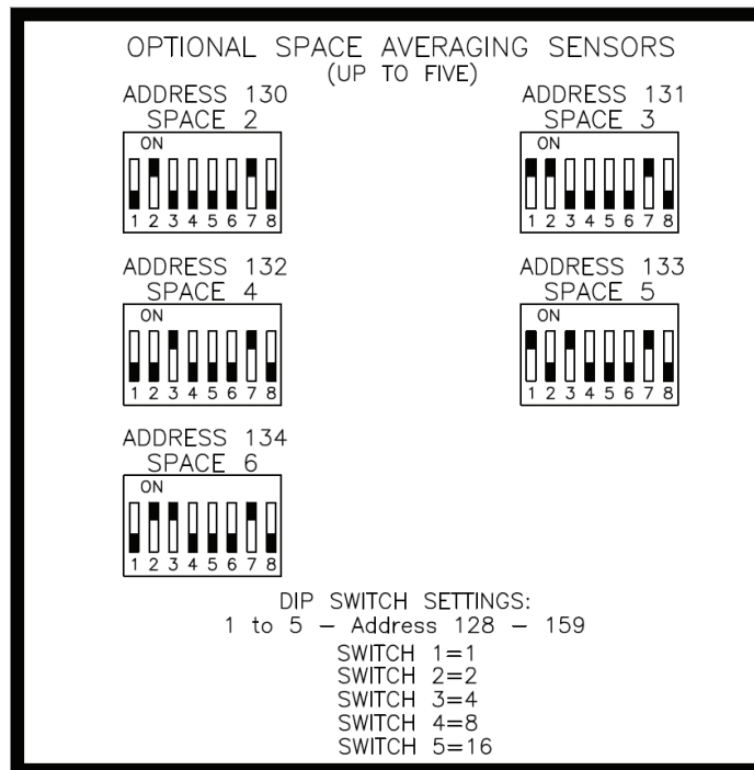
Figure 5. Space Averaging Sensor DIP Switch Settings
