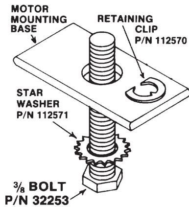
Figure 17. Blower- and Motor-Mounting Components (Refer to Table 24 )
