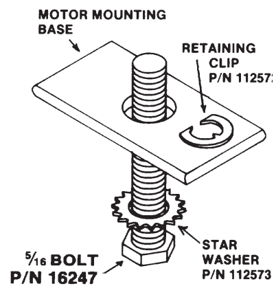
Hardware for 5/16-Inch Motor Mounting Bolts
