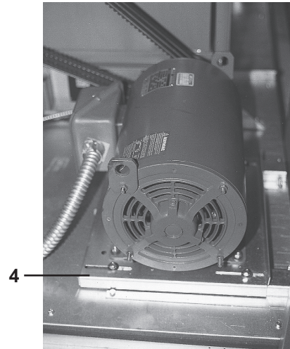
RDF-2 and RDF-3 Blower Motor
