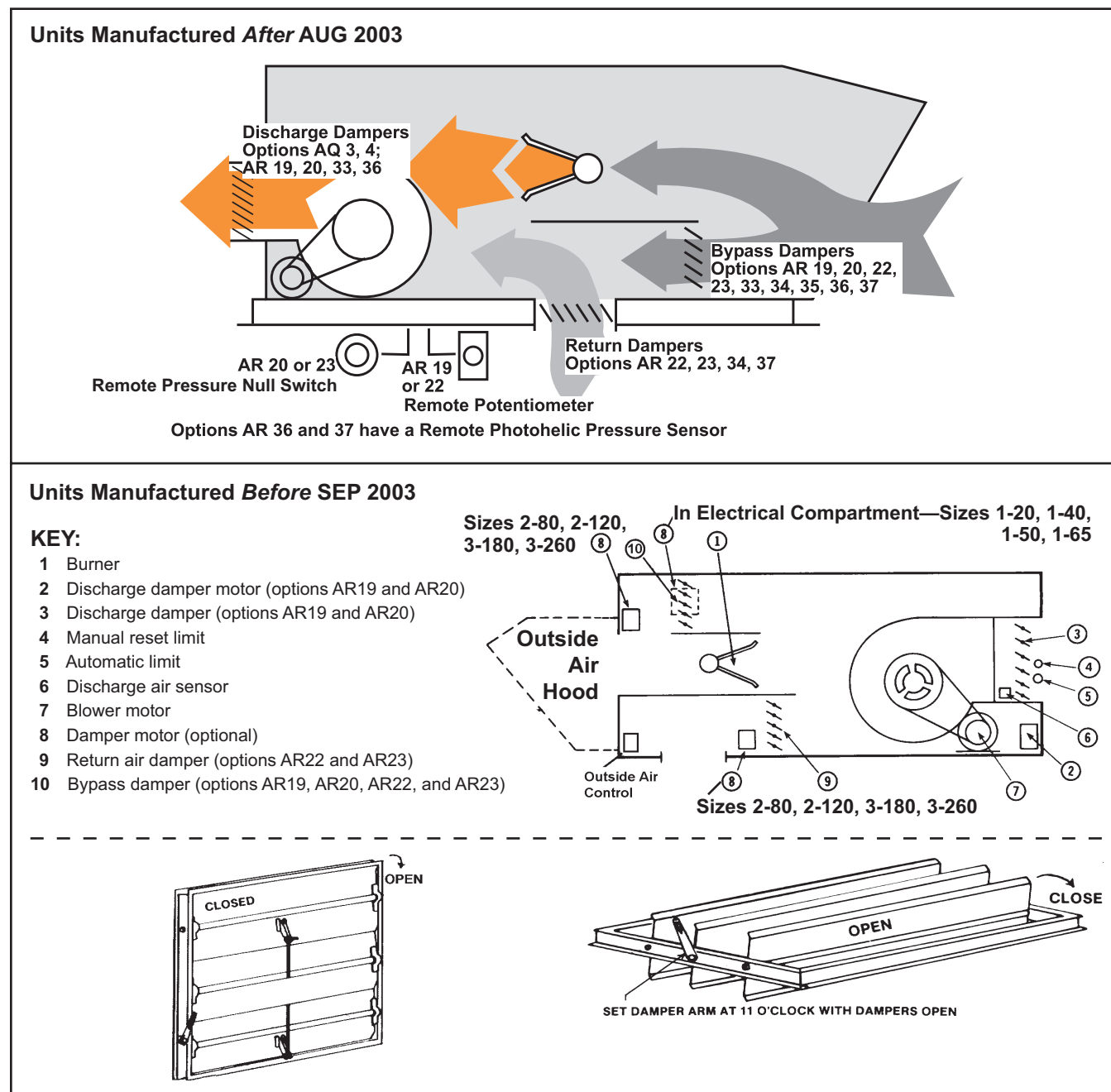
Figure 14. Damper and Damper Control Locations
