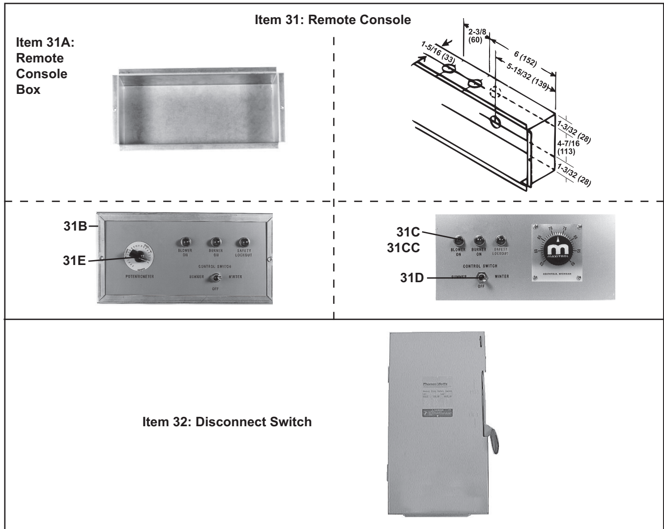
Figure 3. Individual Electrical Components—Items 31 and 32 (Refer to Table 2 )
