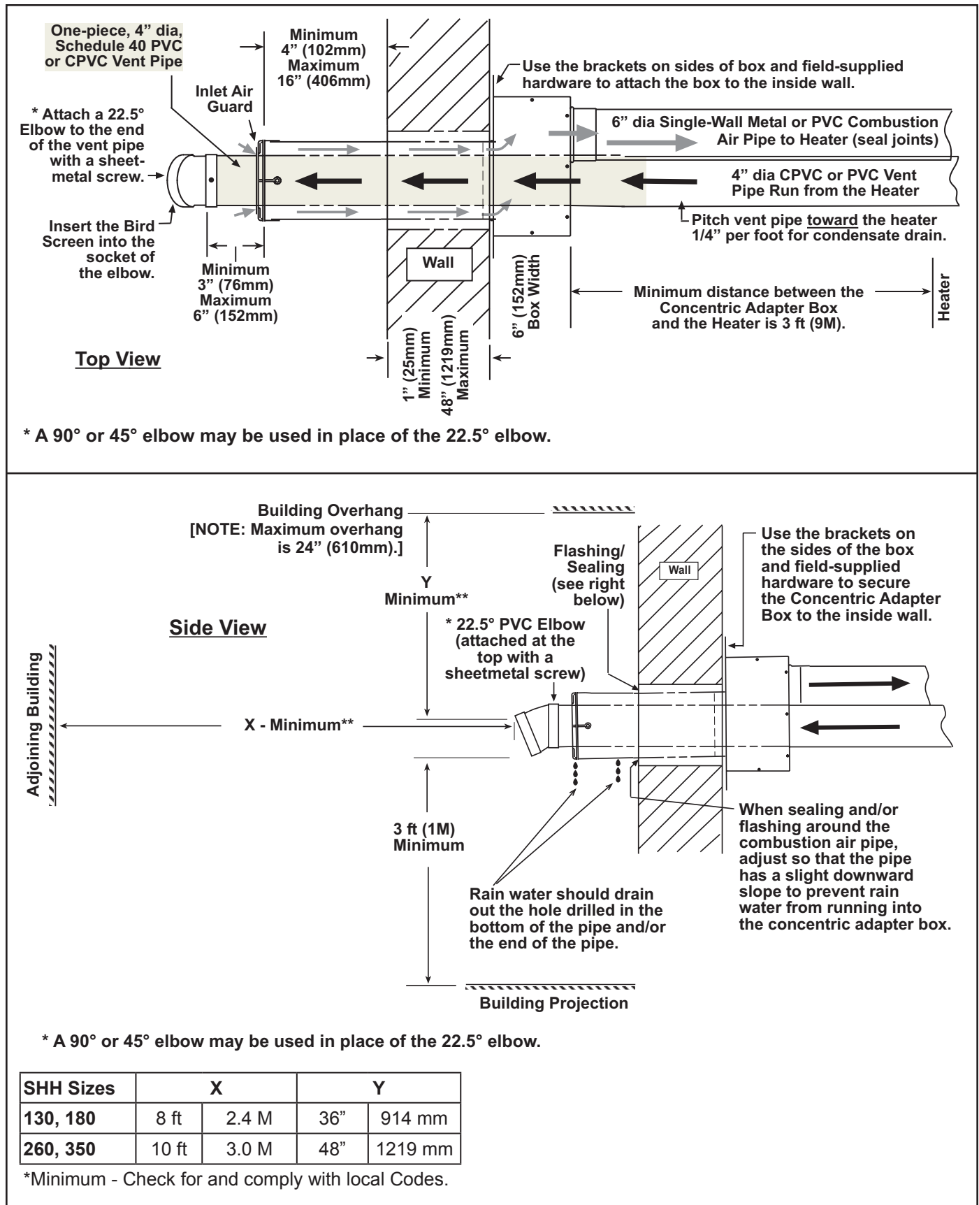
FIGURE 11 - Typical Installation of a Model SHH High Efficiency, Separated-Combustion Unit with a Horizontal Vent/Combustion Air Terminal (Option CC6)
