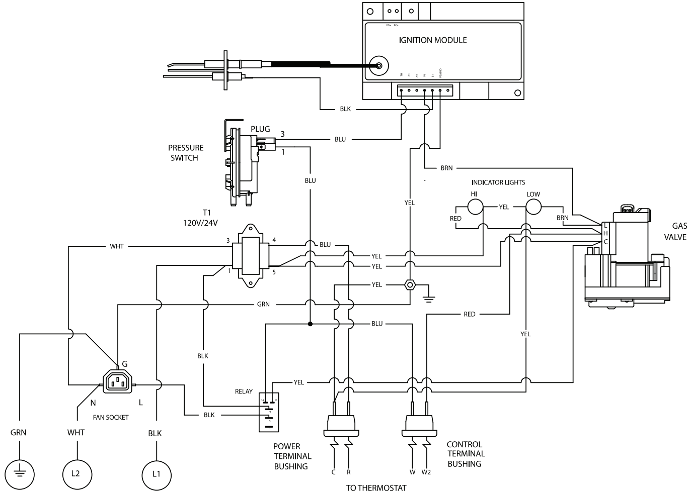
INTERNAL WIRING
