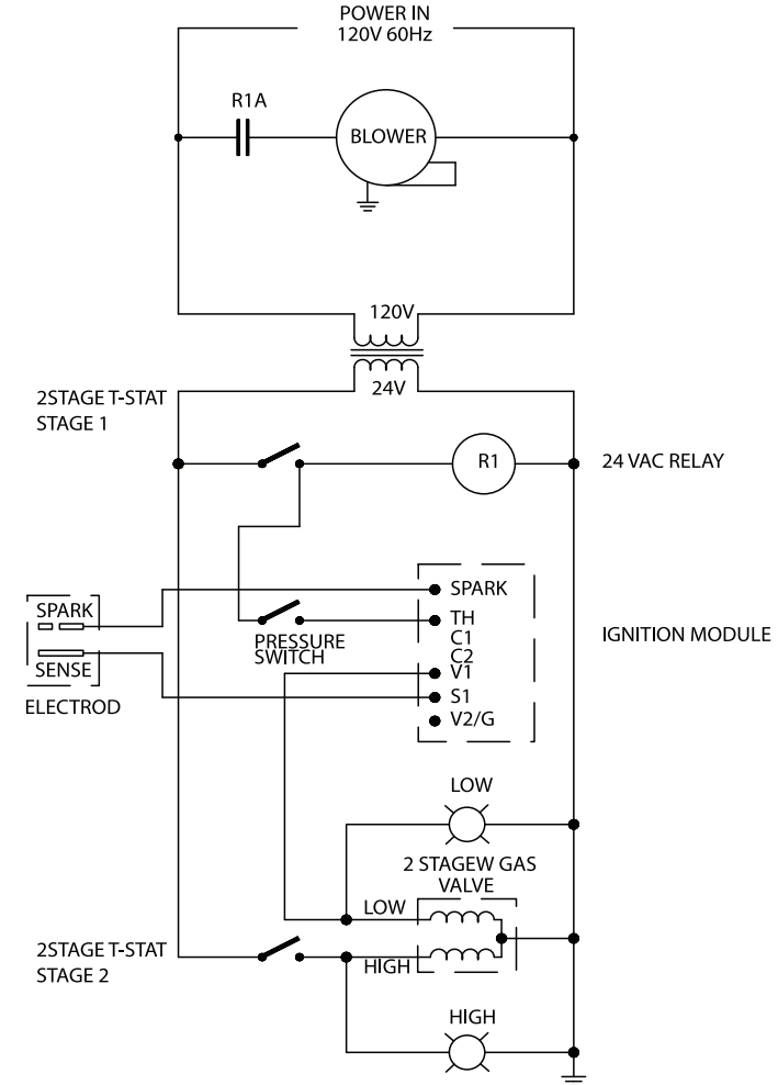
LADDER DIAGRAM
